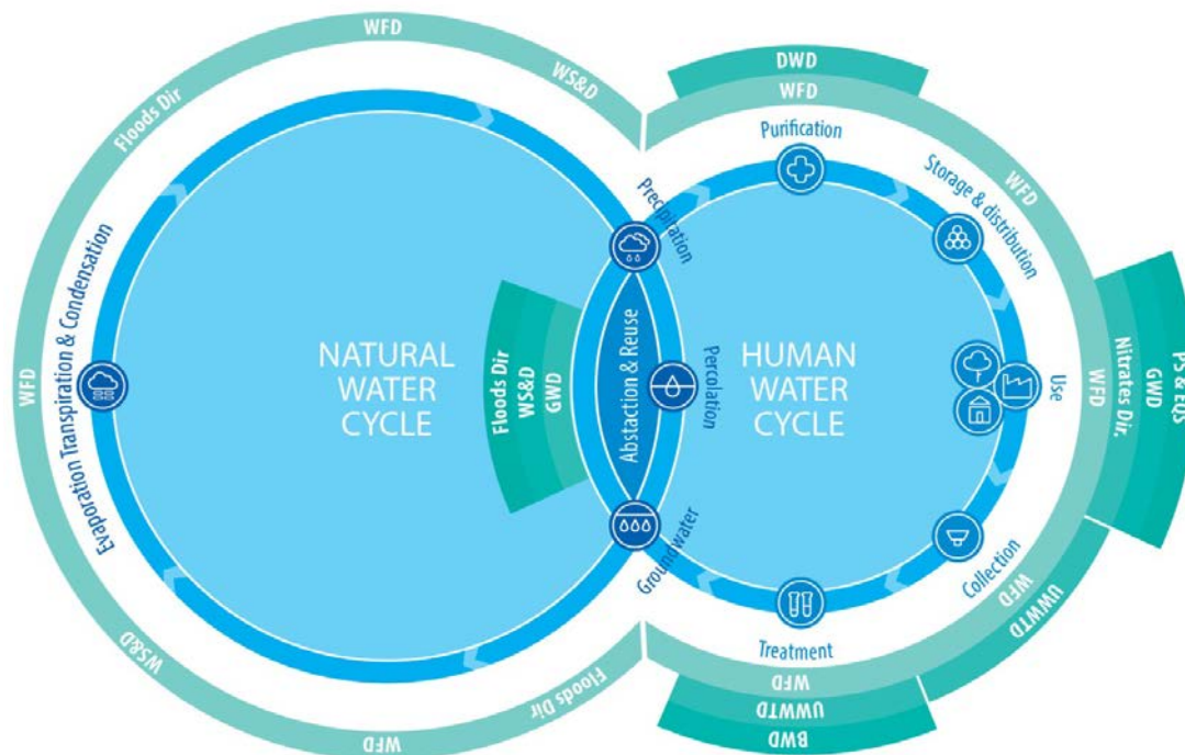
Figure 1: Illustration of the water cycle
